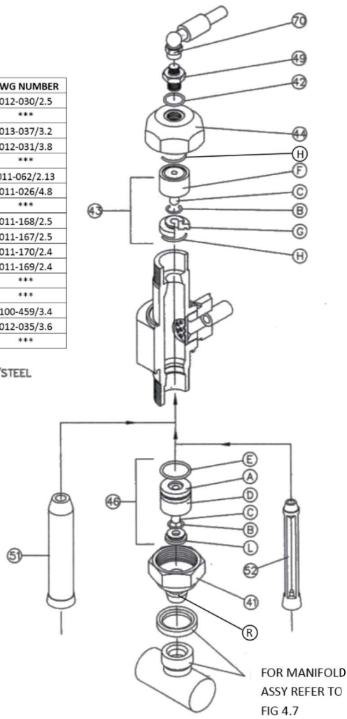
Fig 4.4 'P' Type and High Lift Pump – Barrel Assembly
