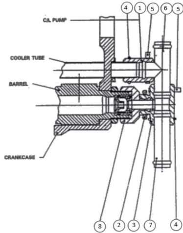
Fig 4.7 'P' Type and High Lift Pump- Inlet Manifold Assembly
