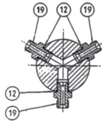
Fig 4.8 Manifold Selector Assembly
